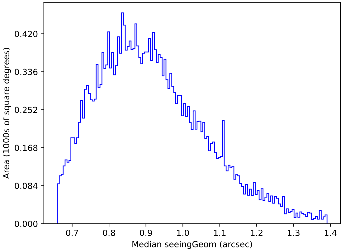
too_ignore_100_1v3.4_10yrs Yr 1 g band: Median seeingGeom
