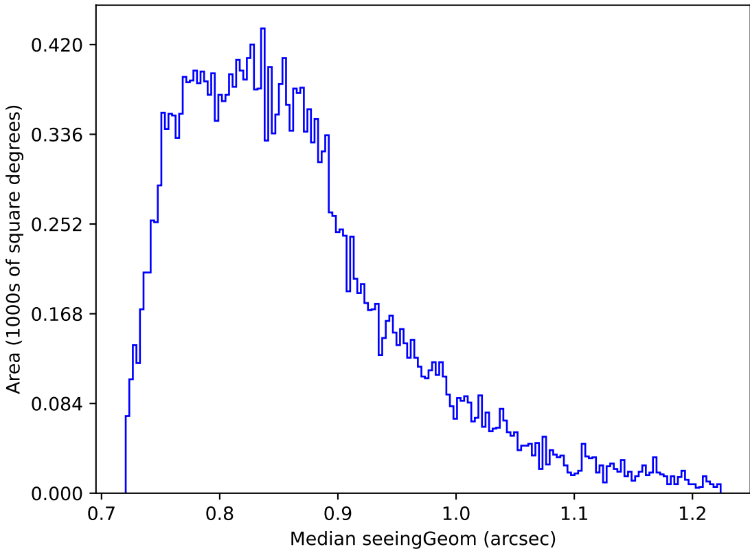
too_ignore_100_1v3.4_10yrs Yr 1 all bands: Median seeingGeom
