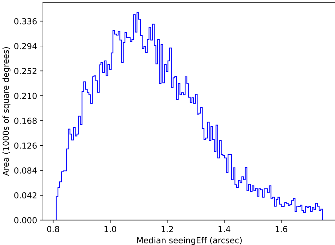
too_ignore_100_1v3.4_10yrs Yr 1 u band: Median seeingEff
