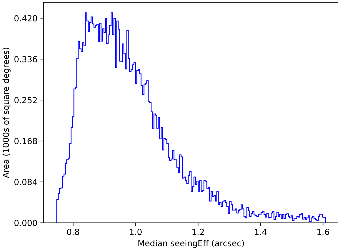
too_ignore_100_1v3.4_10yrs Yr 1 r band: Median seeingEff
