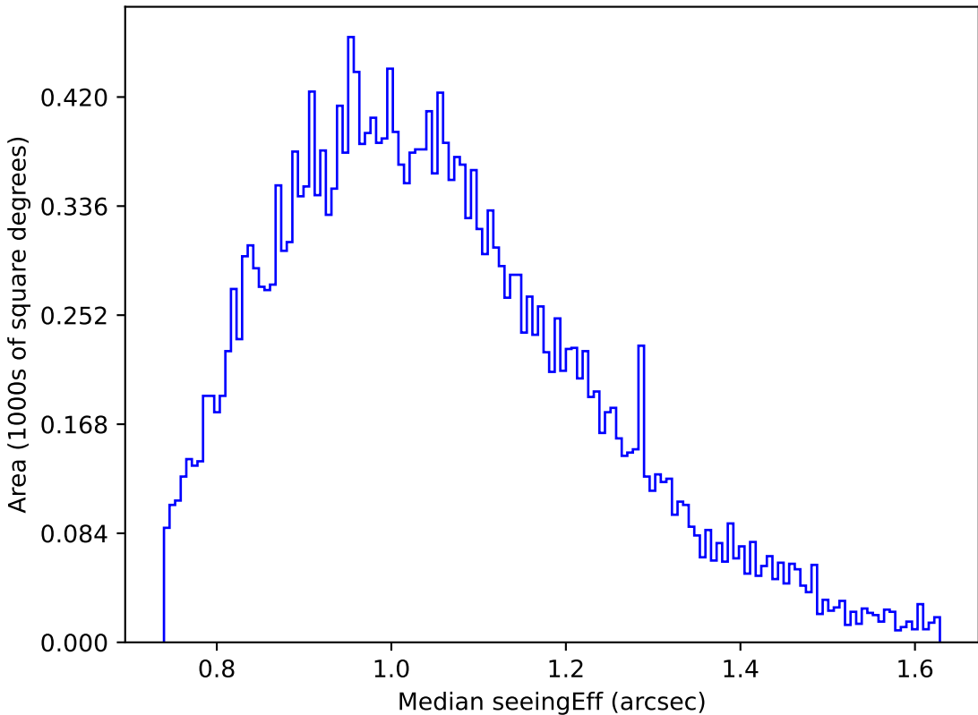
too_ignore_100_1v3.4_10yrs Yr 1 g band: Median seeingEff
