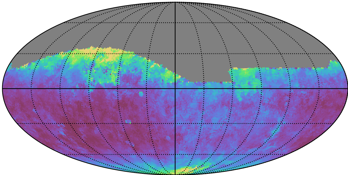
too_ignore_100_1v3.4_10yrs Yr 1 all bands: Median seeingEff
