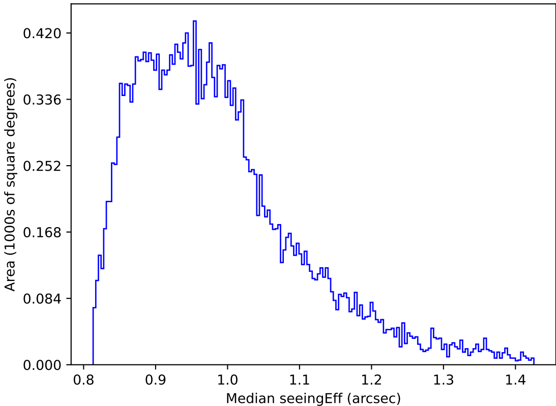
too_ignore_100_1v3.4_10yrs Yr 1 all bands: Median seeingEff
