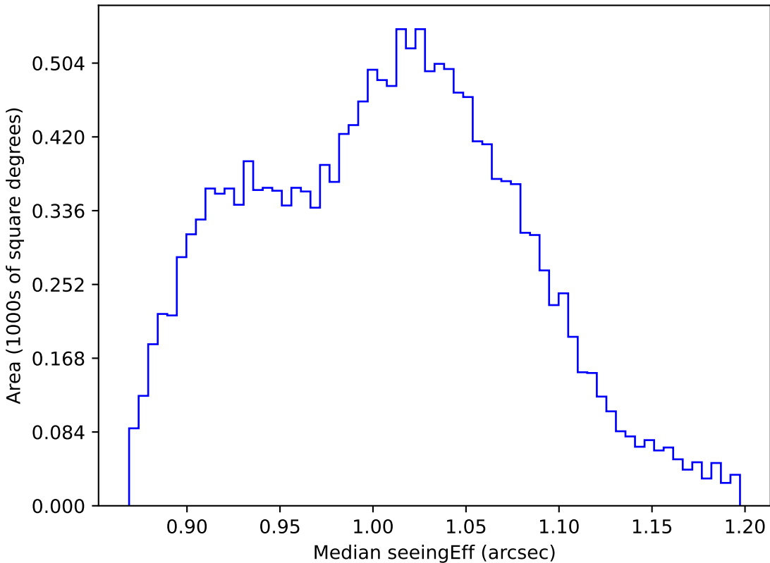
too_ignore_100_1v3.4_10yrs WFD z band: Median seeingEff
