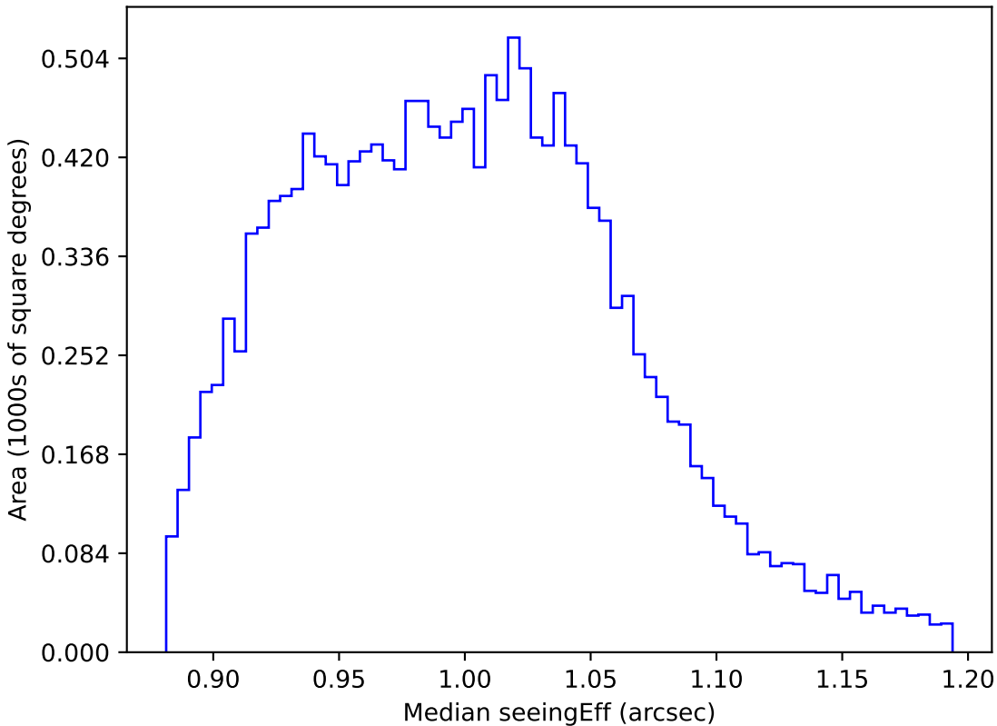
too_ignore_100_1v3.4_10yrs WFD y band: Median seeingEff
