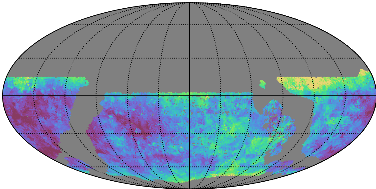
too_ignore_100_1v3.4_10yrs WFD u band: Median seeingEff
