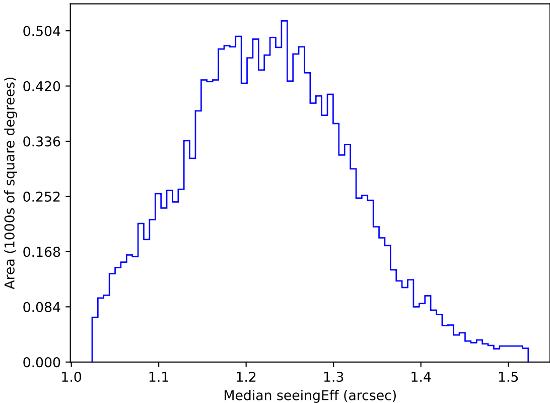
too_ignore_100_1v3.4_10yrs WFD u band: Median seeingEff
