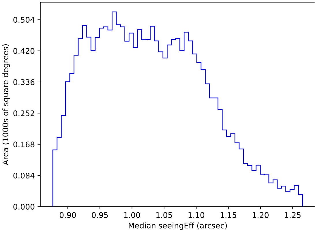
too_ignore_100_1v3.4_10yrs WFD r band: Median seeingEff
