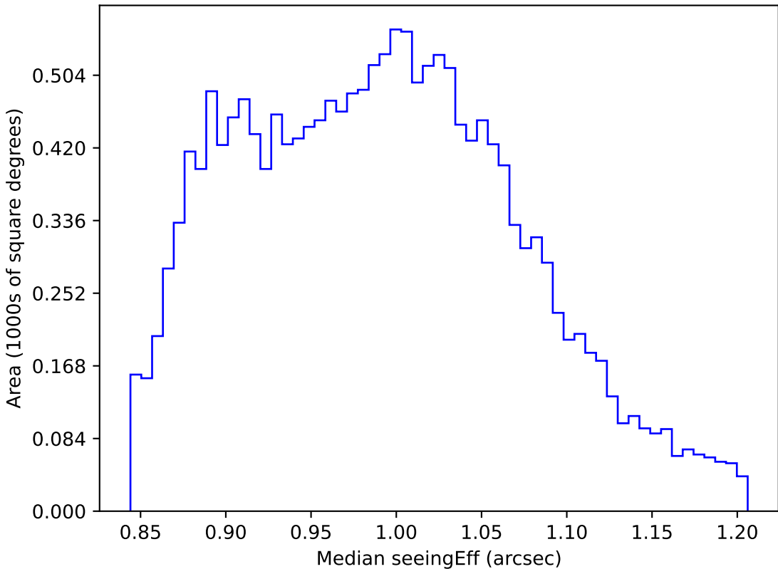
too_ignore_100_1v3.4_10yrs WFD i band: Median seeingEff
