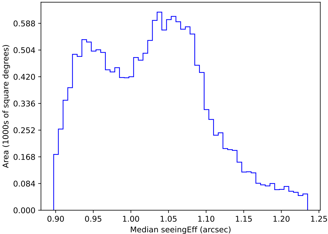
too_ignore_100_1v3.4_10yrs WFD all bands: Median seeingEff
