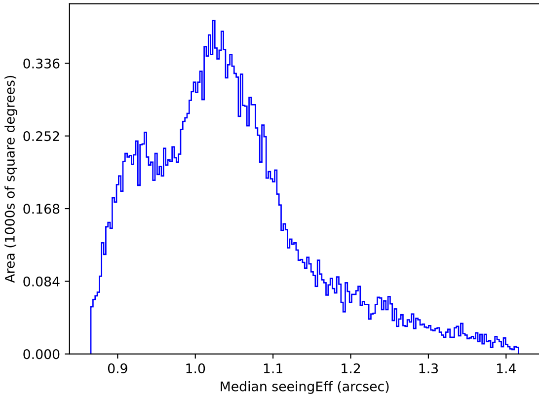
too_ignore_100_1v3.4_10yrs All sky z band: Median seeingEff
