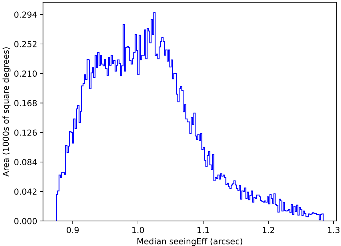
too_ignore_100_1v3.4_10yrs All sky y band: Median seeingEff
