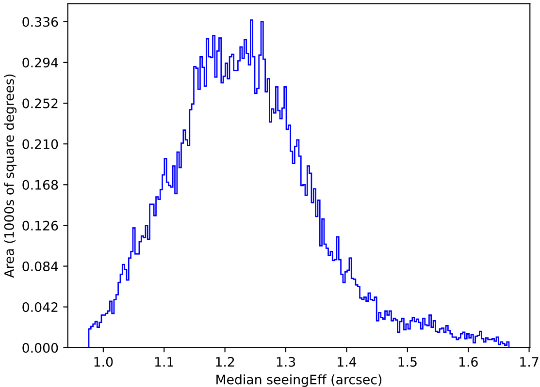
too_ignore_100_1v3.4_10yrs All sky u band: Median seeingEff
