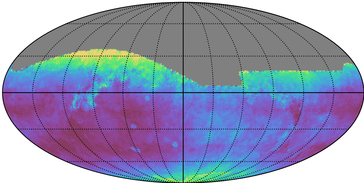
too_ignore_100_1v3.4_10yrs All sky r band: Median seeingEff
