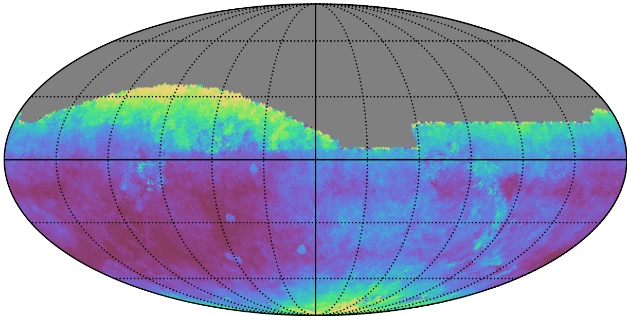
too_ignore_100_1v3.4_10yrs All sky i band: Median seeingEff
