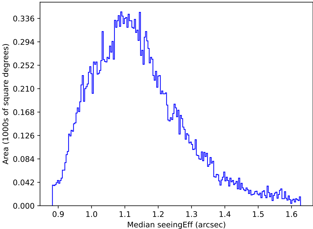
too_ignore_100_1v3.4_10yrs All sky g band: Median seeingEff
