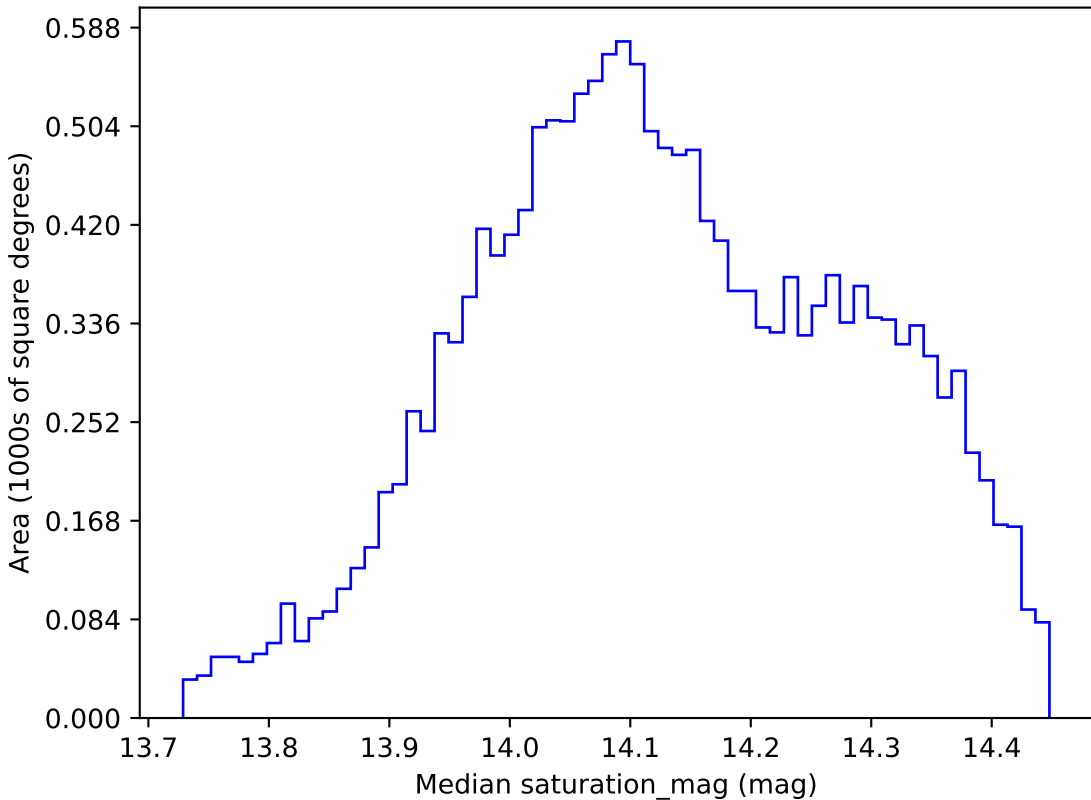
too_ignore_100_1v3.4_10yrs WFD z band: Median saturation_mag
