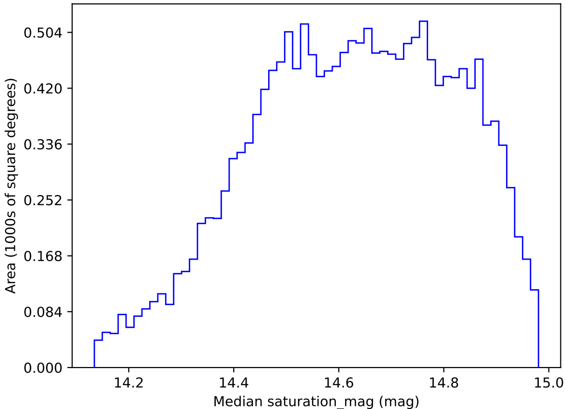
too_ignore_100_1v3.4_10yrs WFD r band: Median saturation_mag
