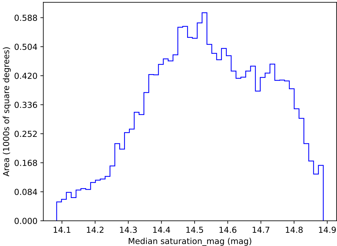
too_ignore_100_1v3.4_10yrs WFD i band: Median saturation_mag
