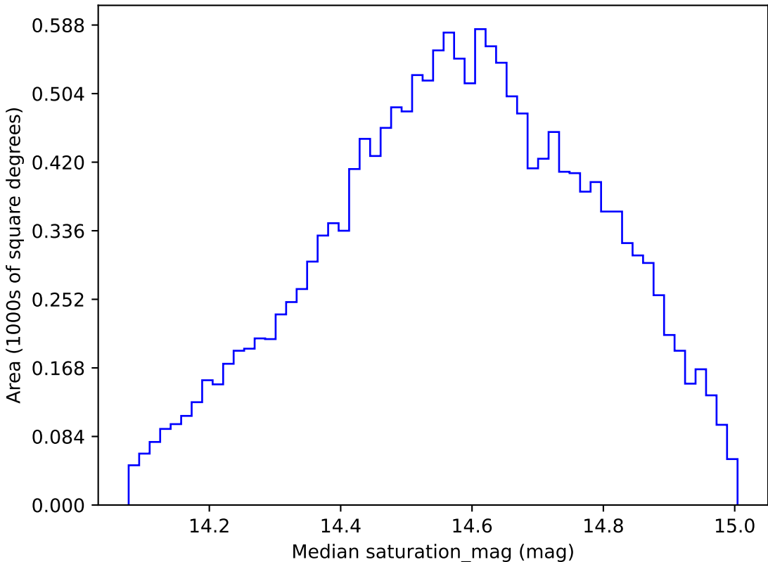
too_ignore_100_1v3.4_10yrs WFD g band: Median saturation_mag
