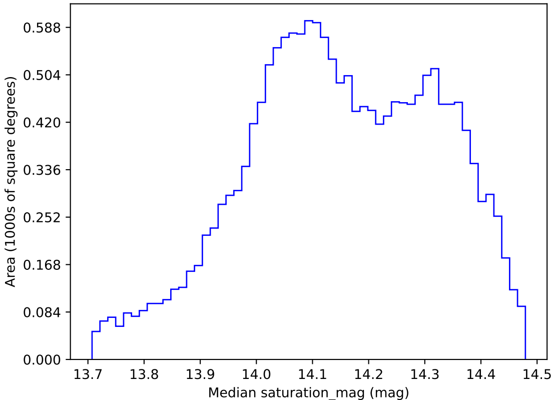
too_ignore_100_1v3.4_10yrs WFD all bands: Median saturation_mag
