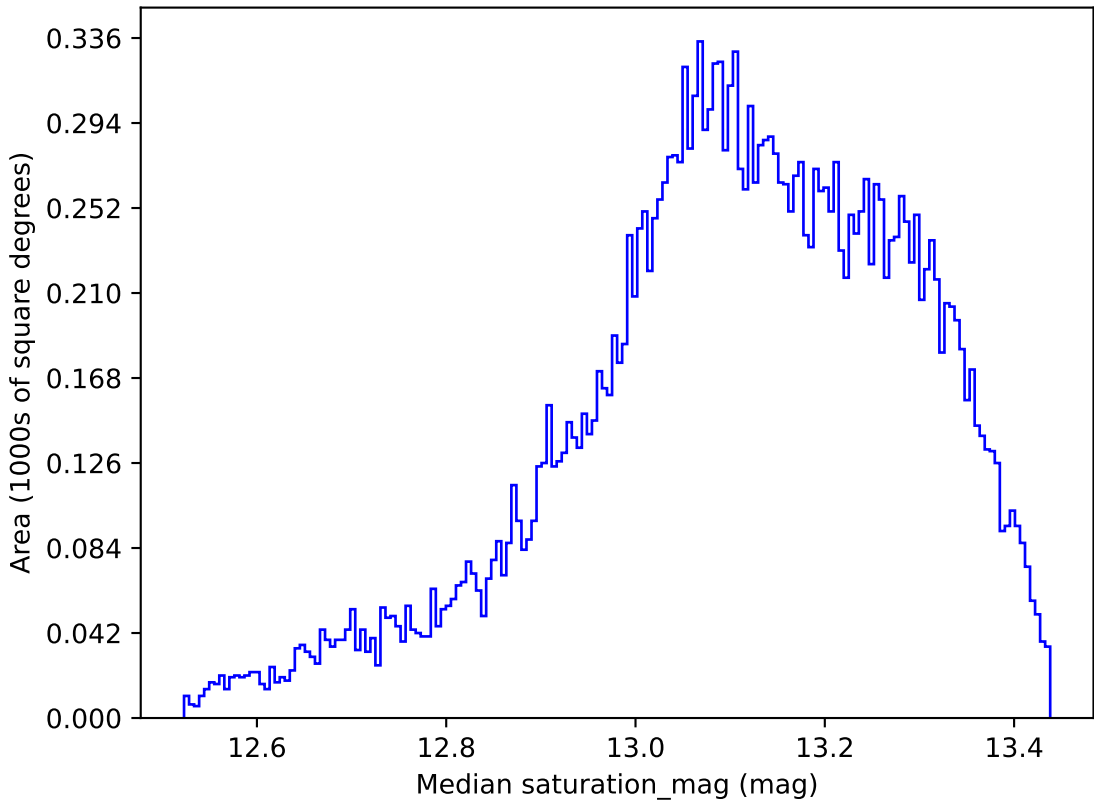
too_ignore_100_1v3.4_10yrs All sky y band: Median saturation_mag
