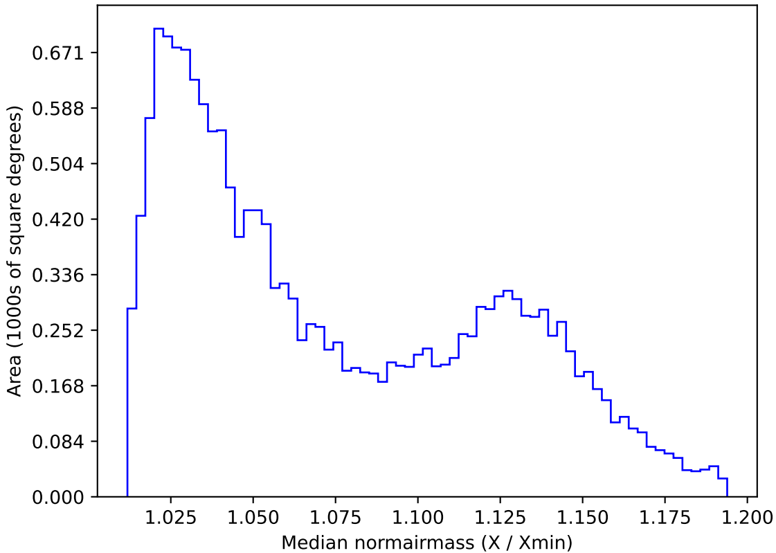
too_ignore_100_1v3.4_10yrs WFD u band: Median normairmass
