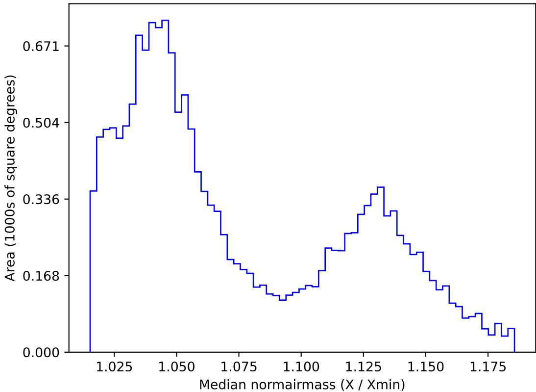
too_ignore_100_1v3.4_10yrs WFD r band: Median normairmass
