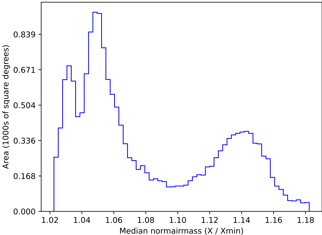
too_ignore_100_1v3.4_10yrs WFD all bands: Median normairmass
