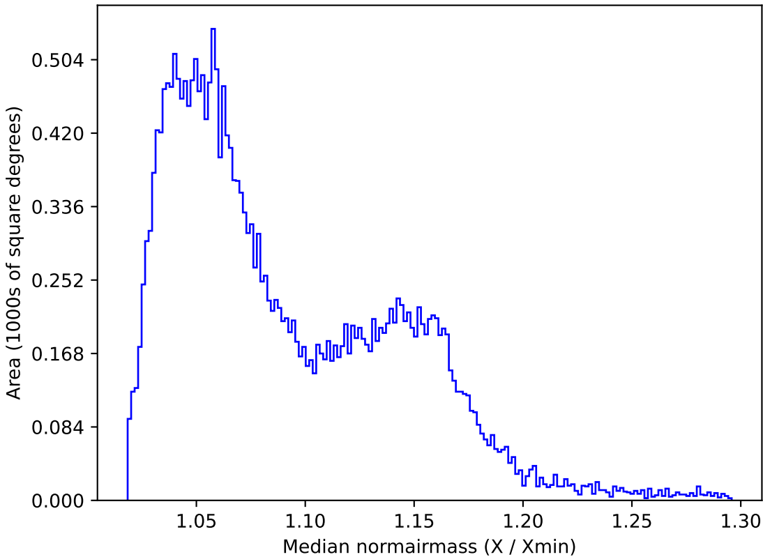
too_ignore_100_1v3.4_10yrs All sky z band: Median normairmass
