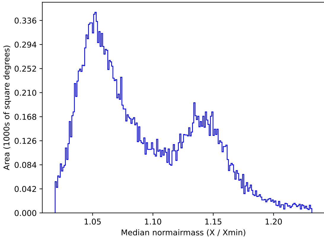
too_ignore_100_1v3.4_10yrs All sky y band: Median normairmass
