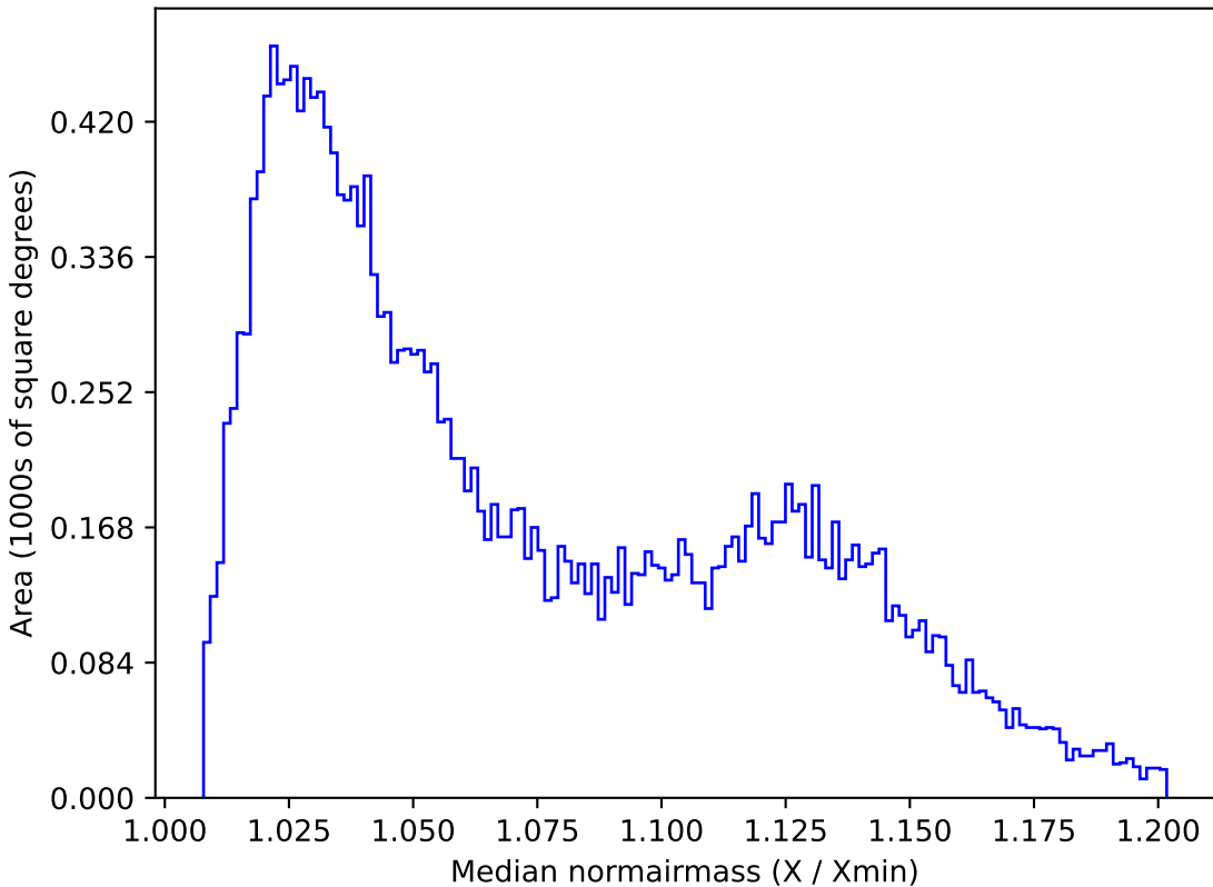
too_ignore_100_1v3.4_10yrs All sky u band: Median normairmass
