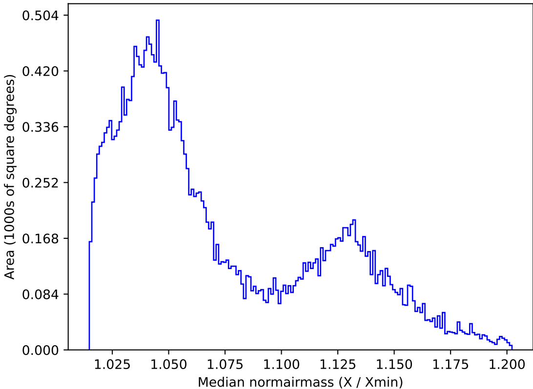
too_ignore_100_1v3.4_10yrs All sky r band: Median normairmass
