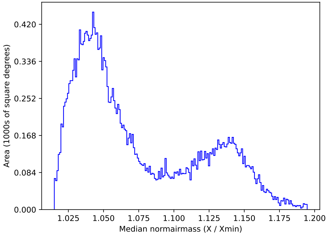
too_ignore_100_1v3.4_10yrs All sky i band: Median normairmass
