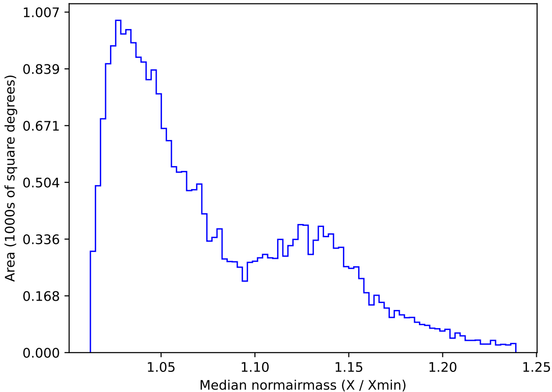
too_ignore_100_1v3.4_10yrs All sky g band: Median normairmass
