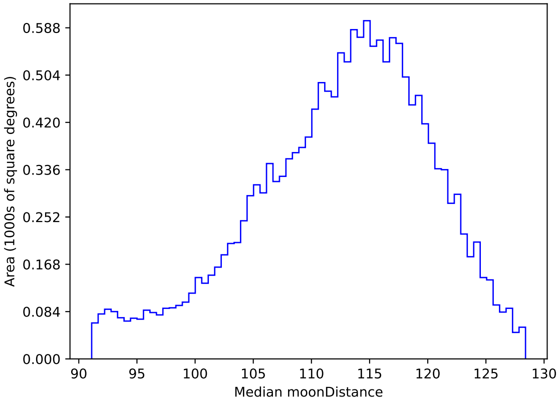
too_ignore_100_1v3.4_10yrs WFD r band: Median moonDistance
