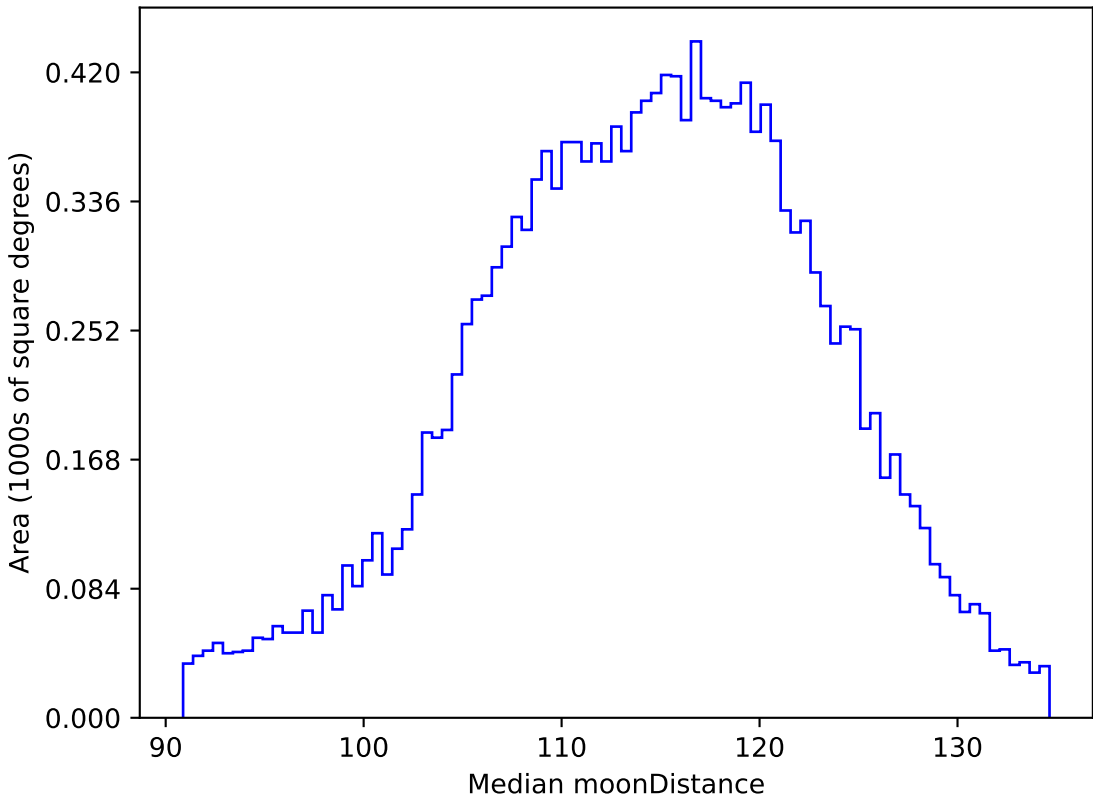
too_ignore_100_1v3.4_10yrs WFD g band: Median moonDistance
