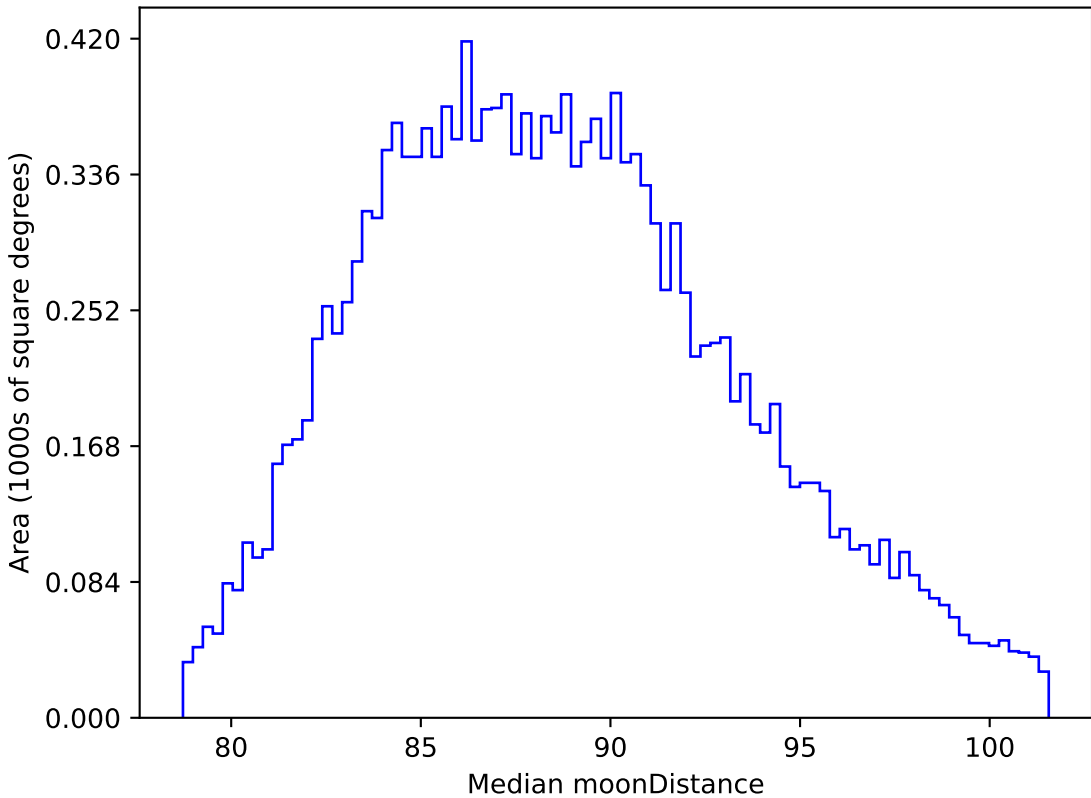
too_ignore_100_1v3.4_10yrs WFD all bands: Median moonDistance
