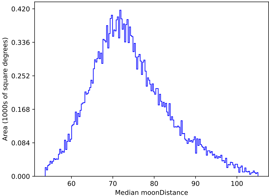
too_ignore_100_1v3.4_10yrs All sky z band: Median moonDistance
