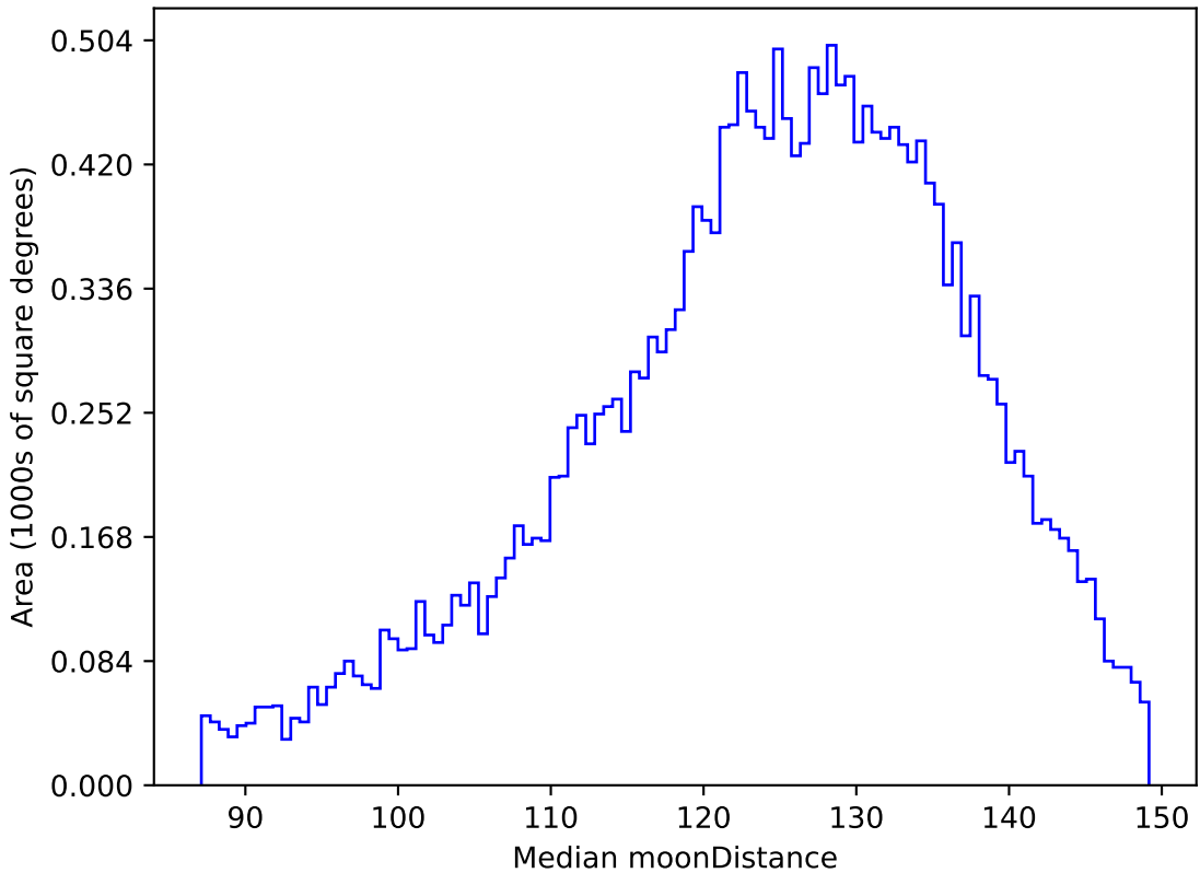
too_ignore_100_1v3.4_10yrs All sky u band: Median moonDistance
