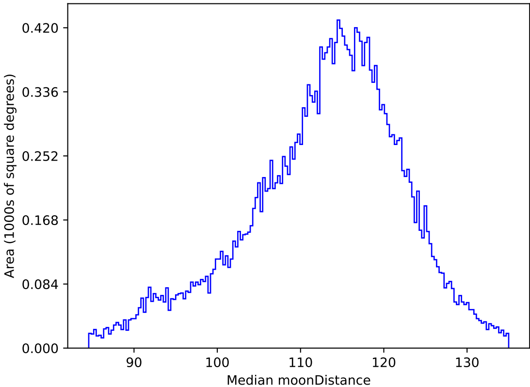
too_ignore_100_1v3.4_10yrs All sky r band: Median moonDistance
