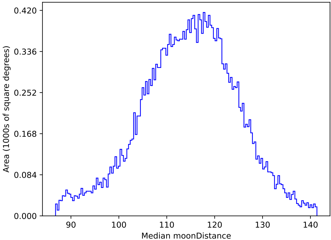
too_ignore_100_1v3.4_10yrs All sky g band: Median moonDistance
