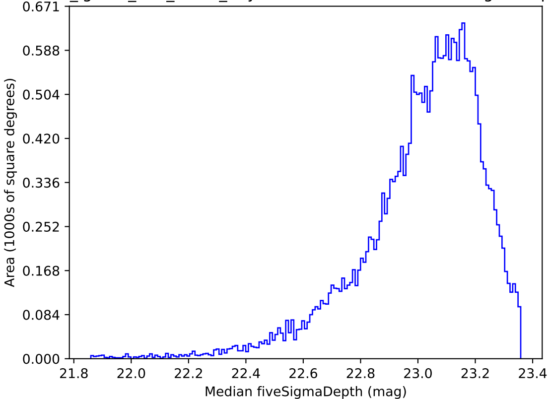
too_ignore_100_1v3.4_10yrs Yr 1 z band: Median fiveSigmaDepth
