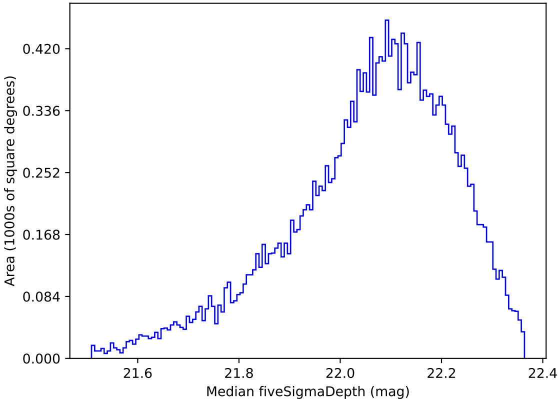
too_ignore_100_1v3.4_10yrs Yr 1 y band: Median fiveSigmaDepth
