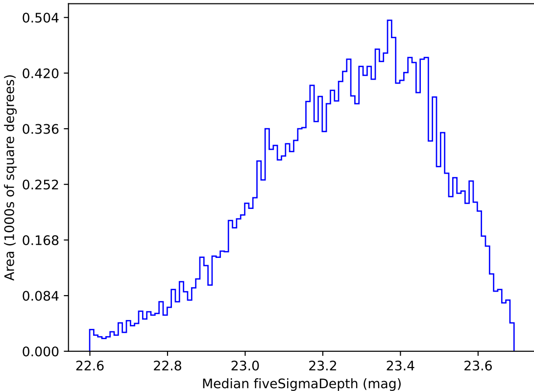
too_ignore_100_1v3.4_10yrs Yr 1 u band: Median fiveSigmaDepth
