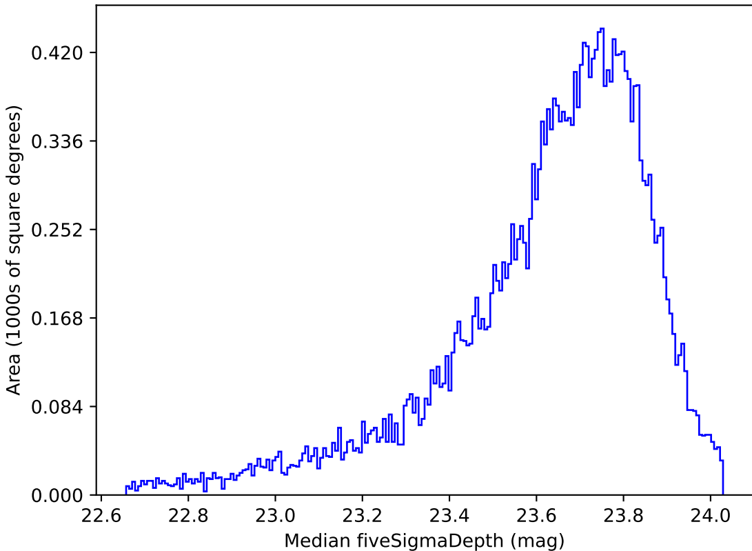
too_ignore_100_1v3.4_10yrs Yr 1 i band: Median fiveSigmaDepth
