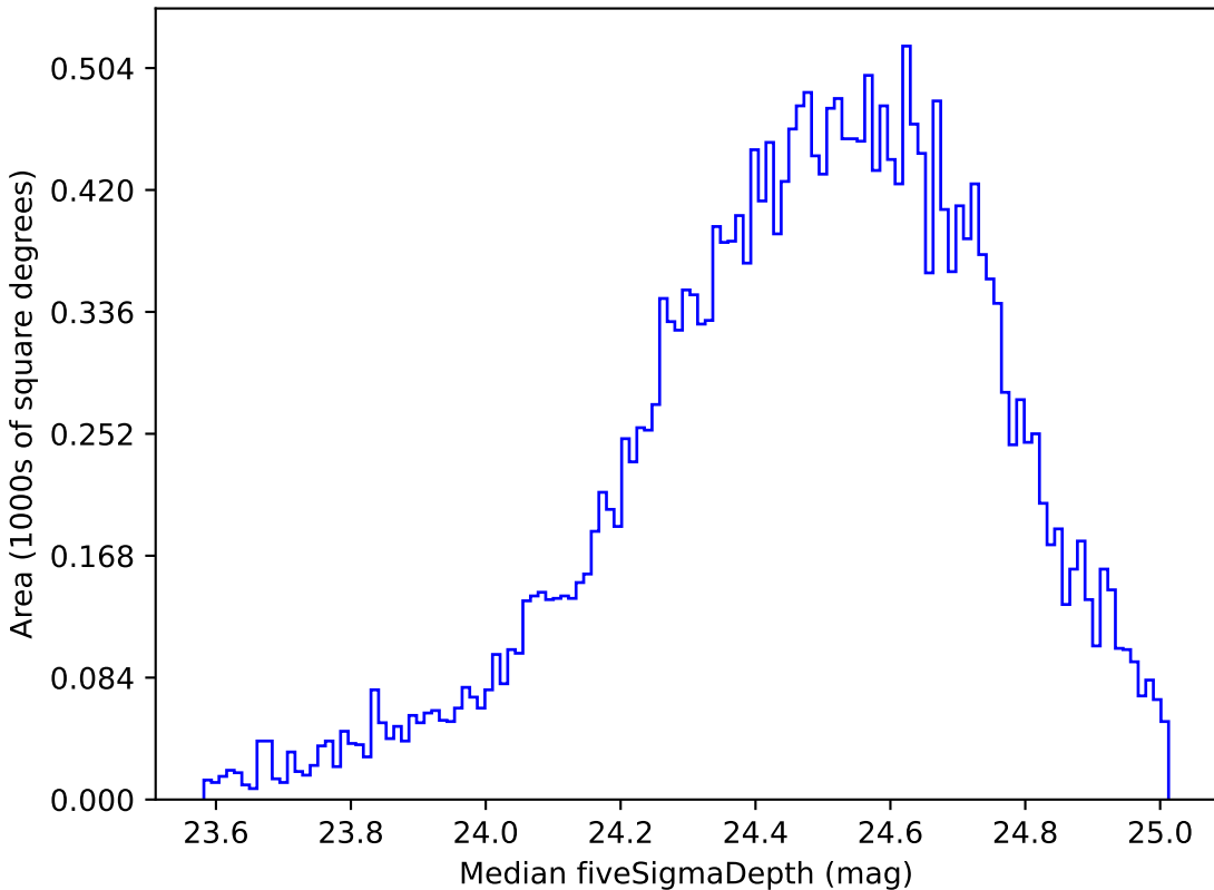
too_ignore_100_1v3.4_10yrs Yr 1 g band: Median fiveSigmaDepth
