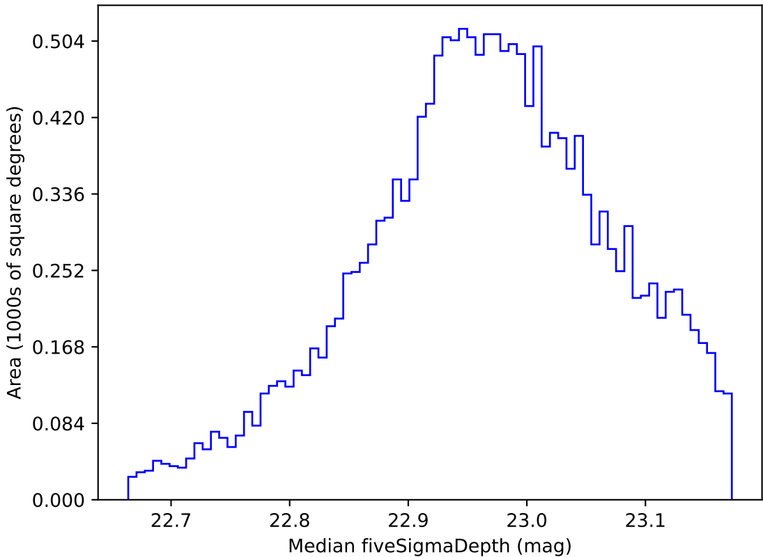
too_ignore_100_1v3.4_10yrs WFD z band: Median fiveSigmaDepth
