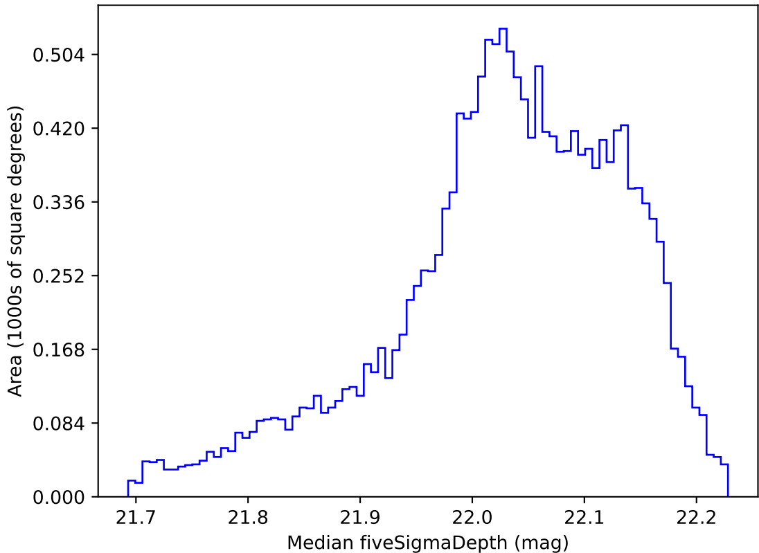
too_ignore_100_1v3.4_10yrs WFD y band: Median fiveSigmaDepth
