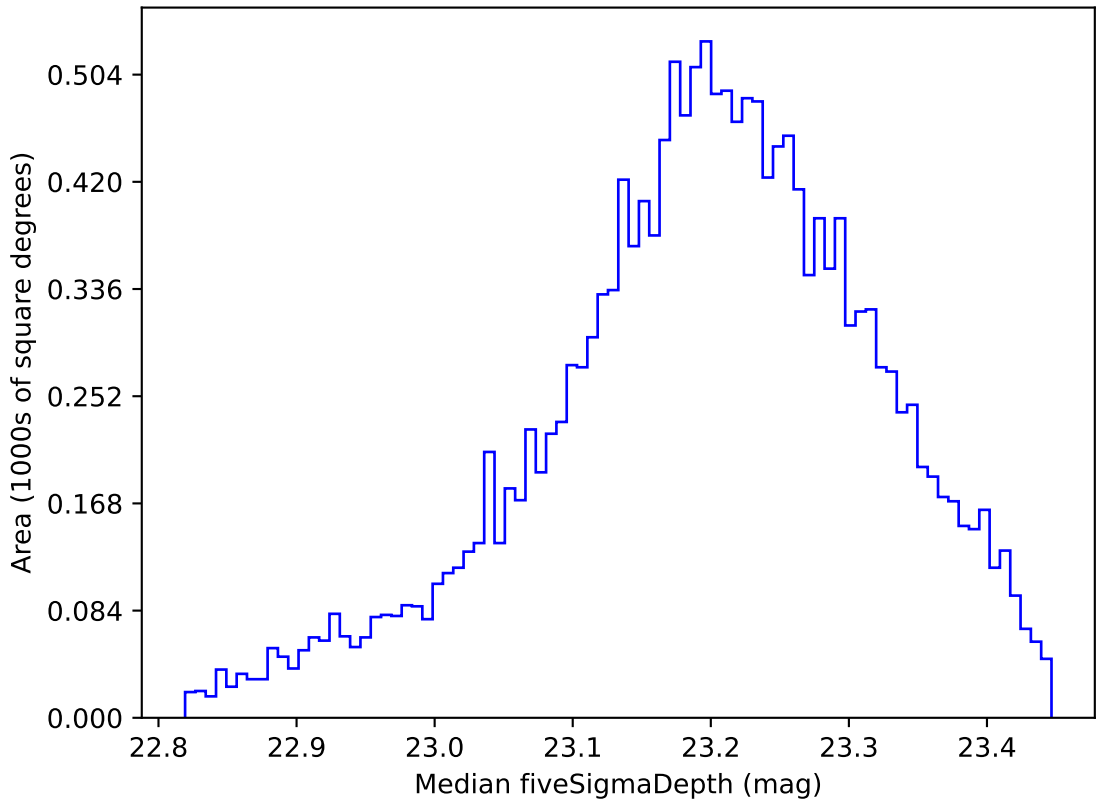
too_ignore_100_1v3.4_10yrs WFD u band: Median fiveSigmaDepth
