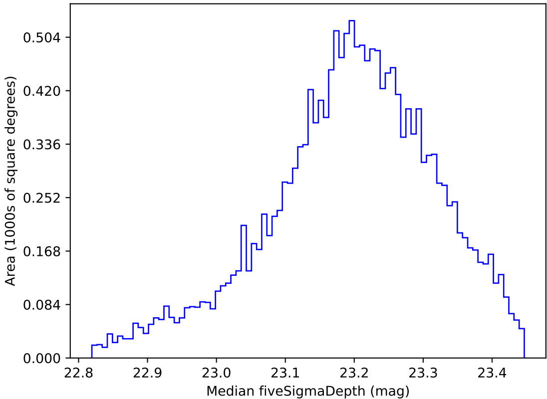
too_ignore_100_1v3.4_10yrs WFD u band: Median fiveSigmaDepth
